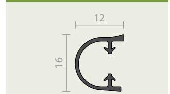
RP394Si BK silicon rubber (SE)
