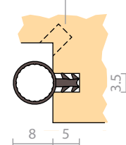
Optional fitting detail
