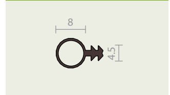
RP331 solid EPDM
