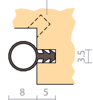
Optional fitting detail
