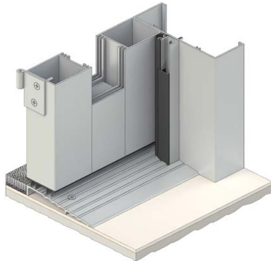
RP84Si RP89 RP77
